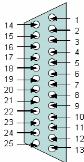
DB25
