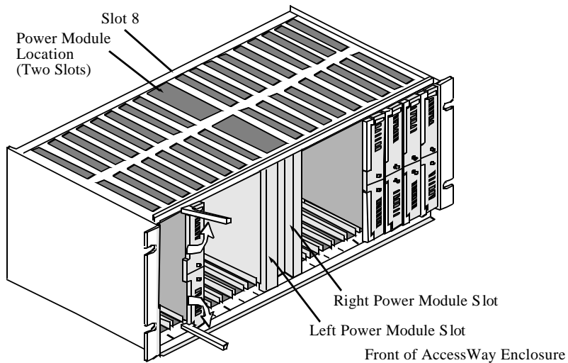
Figure 1. AccessWay Power Module Locations
