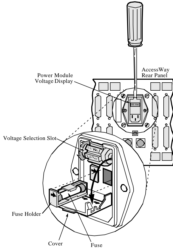
Figure 2. AC Power Module Voltage Selection
